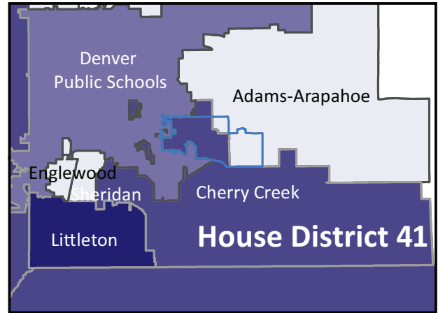
Math
